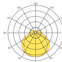
Opal Diffuser
