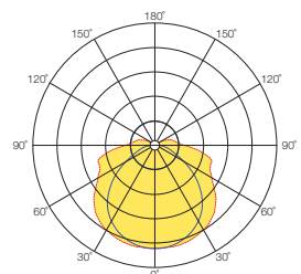
Prismatic Diffuser
