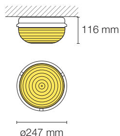
CEILING
