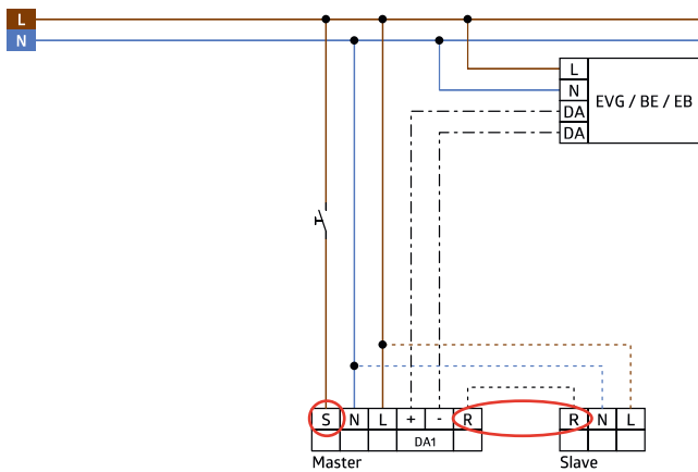
DALI-DSI BROADCAST
