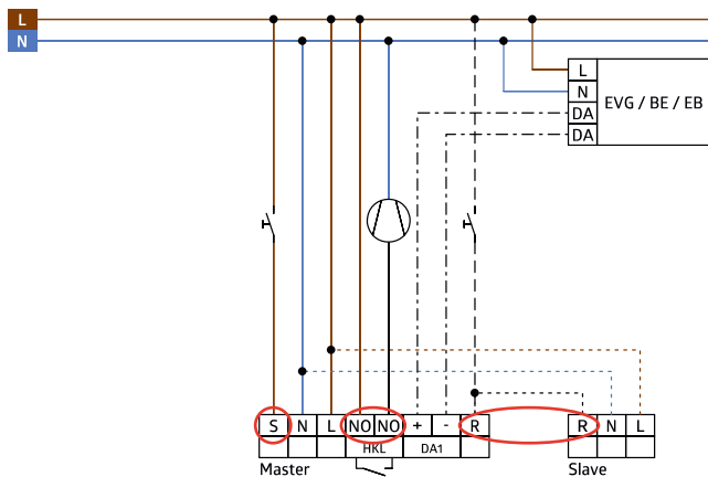
DALI-DSI HKL/HVAC BROADCAST
