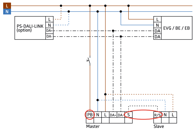
DACO BROADCAST
