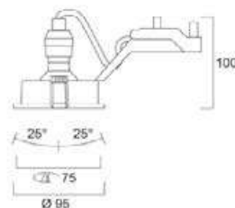
Inset Trend 75 Swing IP44 Interior
