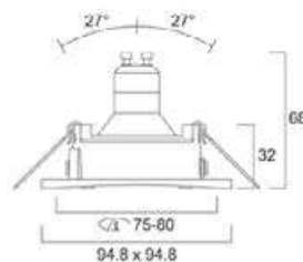
Inset Trend 75 Square IP44 Interior
