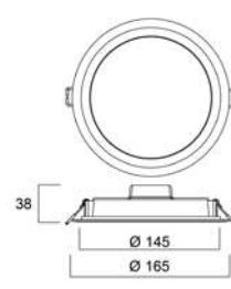
START Downlight Eco 145 round
