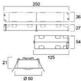
LiFeSafe - Downlight empotrado
