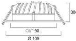
START Downlight 90 IP44
