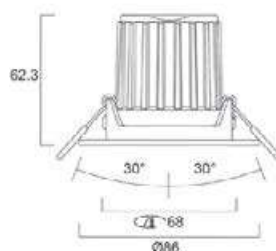
START Spot Alu IP44
