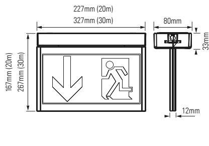
GuideLed 10821 - 20m GuideLed 11821 - 30m
