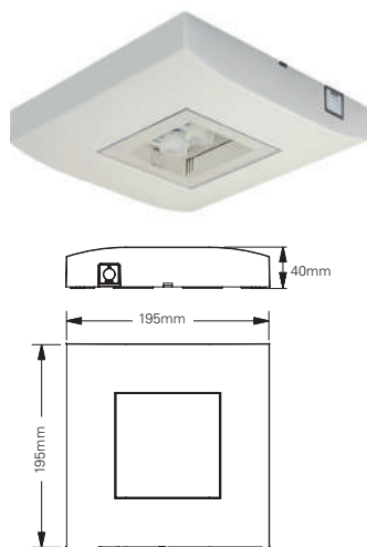
GuideLed SL 13852 CGLine+
