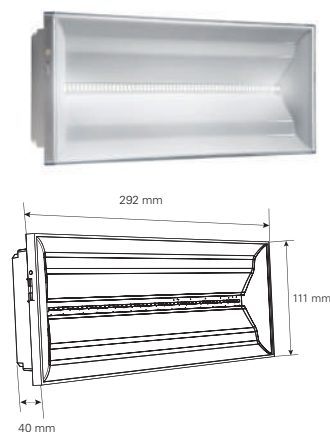
NexiTech LEDTM CGLine+ IP40
