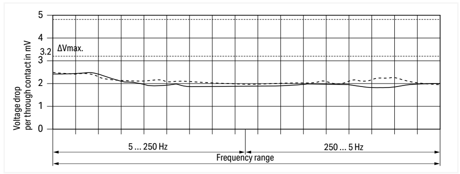
Frequency cycle Rail-mount terminal block: Item no. 280-681 Test current: 1/10 I N = 2,4 A ----- Test specimen no. 1 - - - - - Test specimen no. 2
