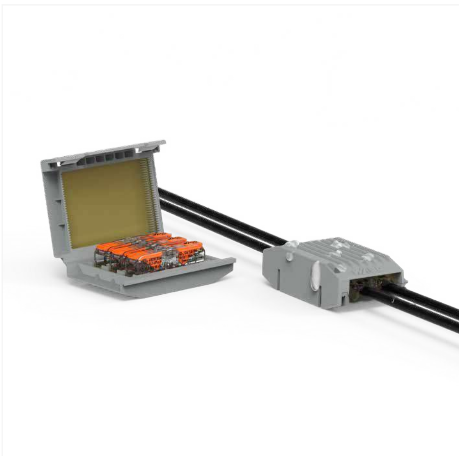
Re-accessible: Open the Gelbox, remove the gel, open the connector and rewire with new components.
