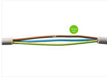
Strip the damaged cable approx. 10 cm uniformly around the damaged area.
